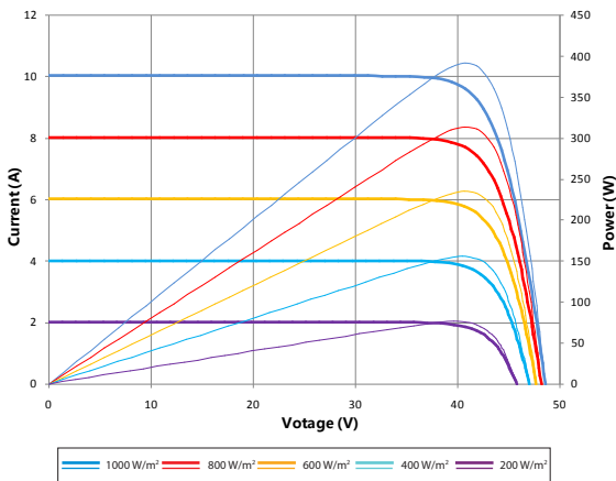
Current-Voltage & Power-Voltage Curve (390S)
