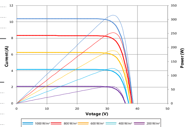
Current-Voltage & Power-Voltage Curve (340S)
