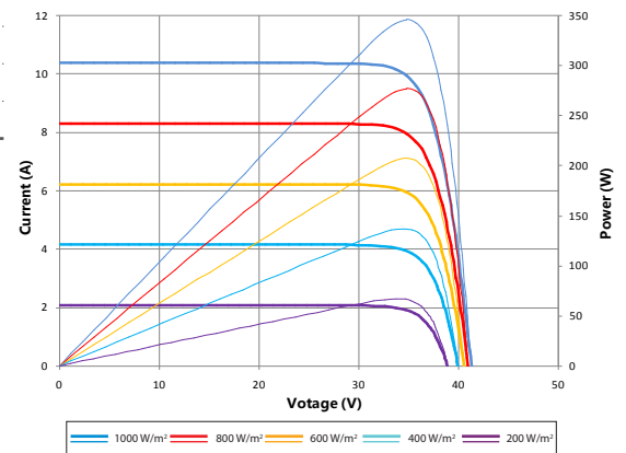
Current-Voltage & Power-Voltage Curve (345S)
