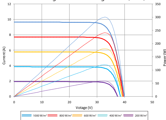
Current-Voltage & Power-Voltage Curve (300S)
