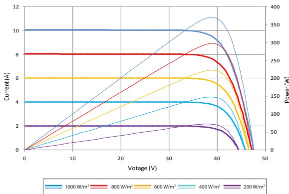
Current-Voltage & Power-Voltage Curve (370S)
