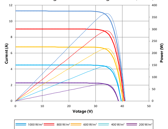
Current-Voltage & Power-Voltage Curve (370S)
