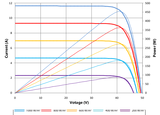
Current-Voltage & Power-Voltage Curve (450S)
