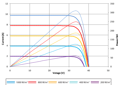
Current-Voltage & Power-Voltage Curve (310S)
