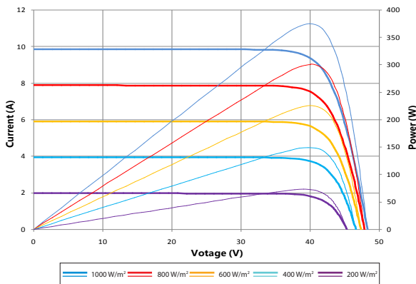
Current-Voltage & Power-Voltage Curve (375S)
