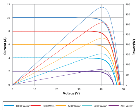
Current-Voltage & Power-Voltage Curve (385S)
