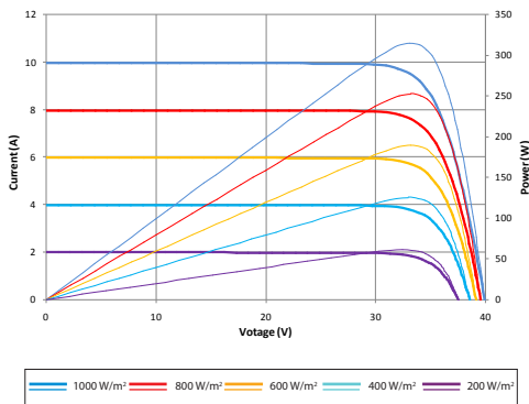
Current-Voltage & Power-Voltage Curve (315S)
